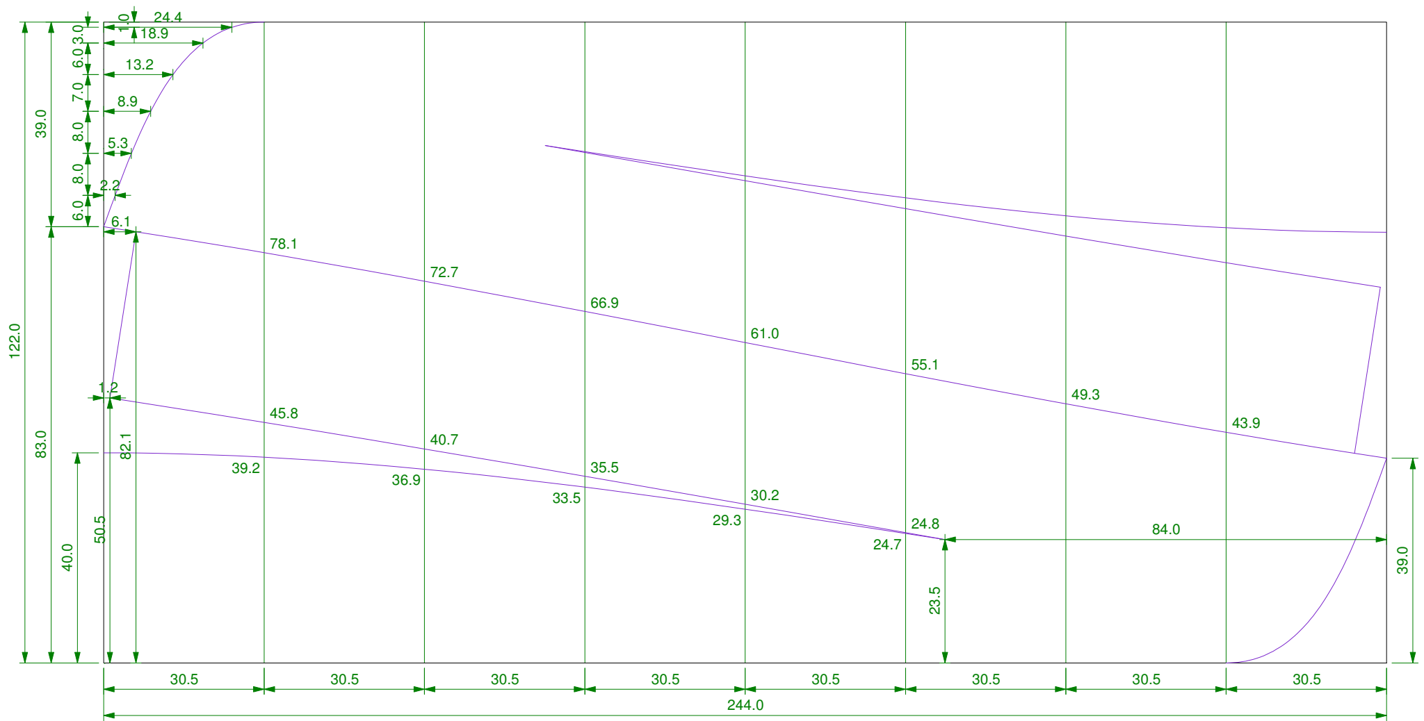
Two sheet Flywood Rowboat - offsets for the panels
